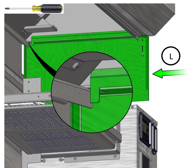
Remove The Corner Rear Screw. Slide (L) Up Into Hood End Opening (See TIP Before Installing)
