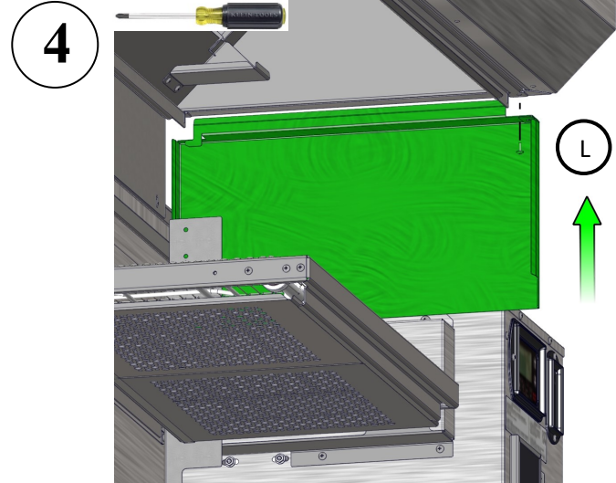
Remove The Corner Rear Screw. Slide (L) Up Into Hood End Opening (See TIP Before Installing)
