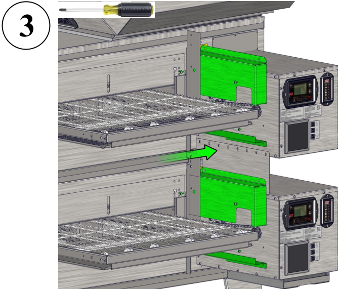
Re-Install Upper & Lower Chain Guards
