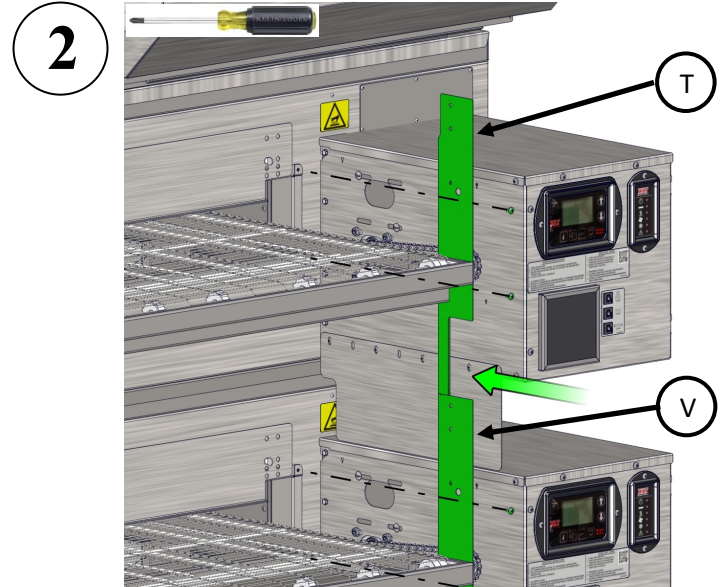
Install (T) & (V) Using Existing Oven Bezel Screws (See TIP before installing)
