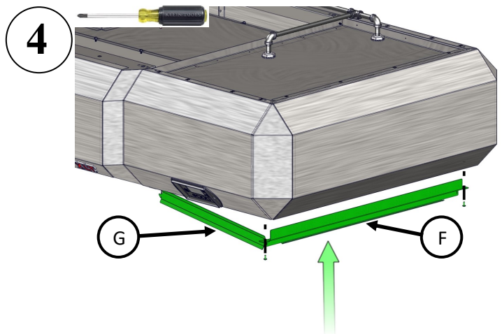
Remove Screws Noted
