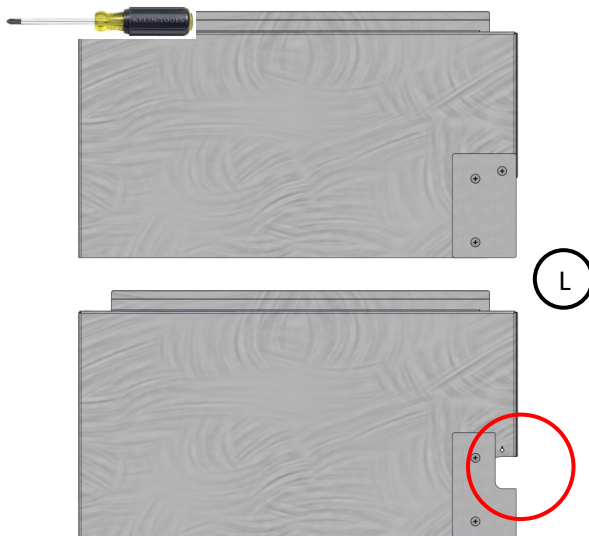
Re-Install Upper & Lower Chain Guards
